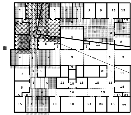
Figure 4: Object lookahead set computation.
