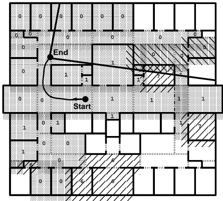
Figure 6: Cells containing resident objects (stipple), read objects (left-hatch), and released objects (right-hatch).
