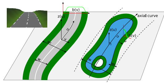
Figure 7: Z-profiles and blending profiles are based on the (u, v) coordinates of the strip. Top left inset: b(v) gives smooth roadsides.
